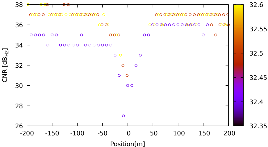
CNR vs position for G19 (L1) on HuaweiP40 - DOY 263 jam. 3
