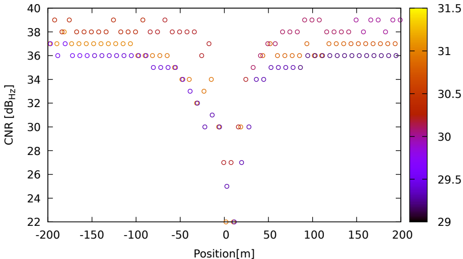
CNR vs position for G21 (L1) on HuaweiP40 - DOY 263 jam. 1
