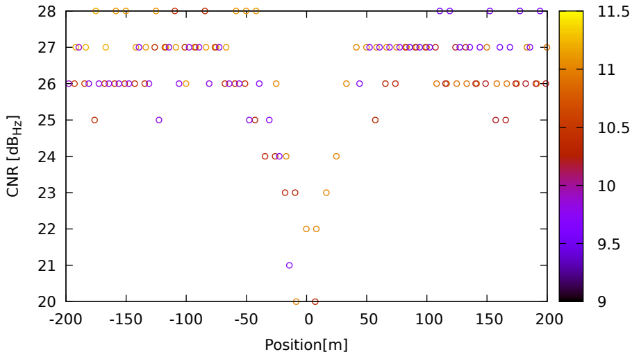
CNR vs position for G22 (L1) on HuaweiP40 - DOY 263 jam. 3
