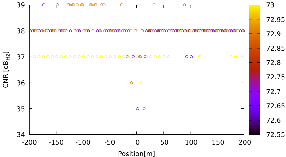
CNR vs position for R02 (G1) on HuaweiP40 - DOY 263 jam. 2
