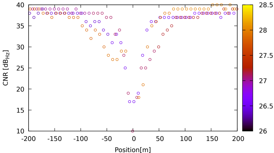
CNR vs position for R03 (G1) on HuaweiP40 - DOY 263 jam. 1
