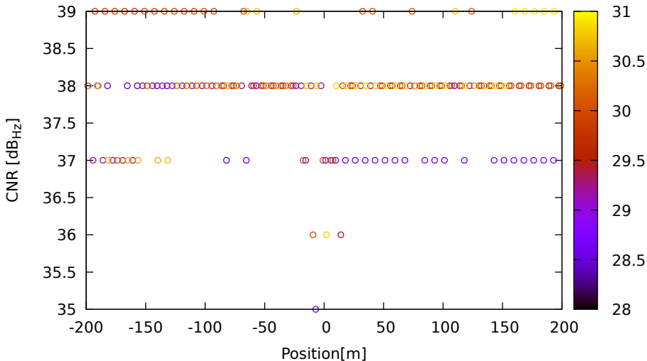
CNR vs position for R03 (G1) on HuaweiP40 - DOY 263 jam. 2
