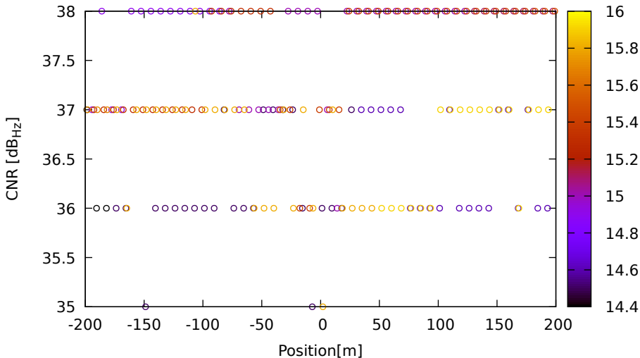
CNR vs position for R11 (G1) on HuaweiP40 - DOY 263 jam. 2
