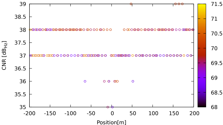
CNR vs position for R17 (G1) on HuaweiP40 - DOY 263 jam. 2
