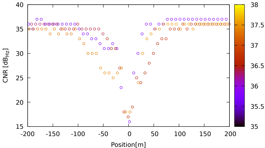
CNR vs position for R18 (G1) on HuaweiP40 - DOY 263 jam. 1
