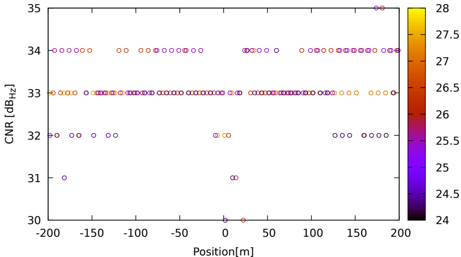
CNR vs position for R24 (G1) on HuaweiP40 - DOY 263 jam. 2
