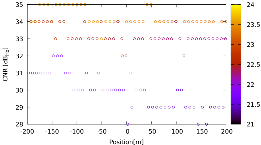
CNR vs position for R24 (G1) on HuaweiP40 - DOY 263 jam. 3
