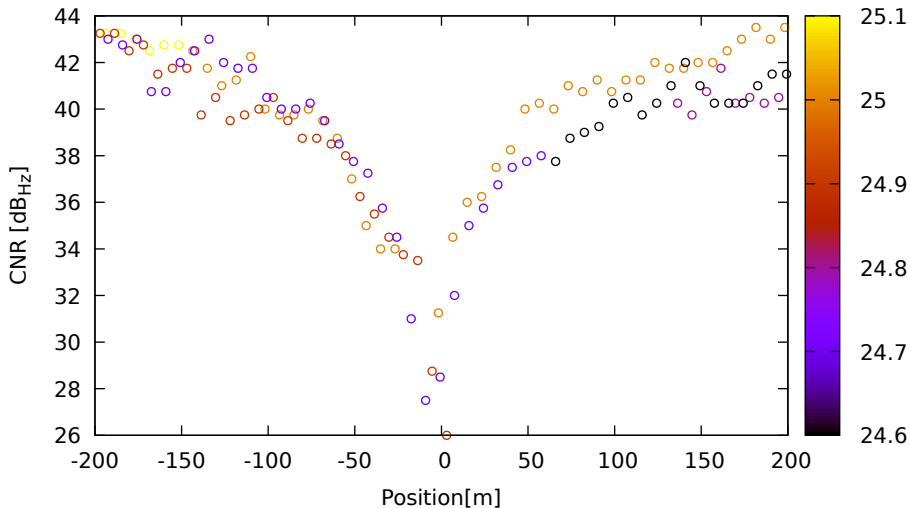
CNR vs position for C06 (B2) on LeicaGS18 - DOY 263 jam. 1
