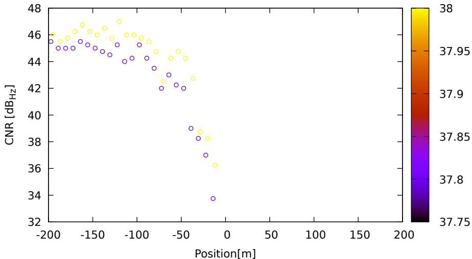
CNR vs position for C09 (B1) on LeicaGS18 - DOY 263 jam. 2
