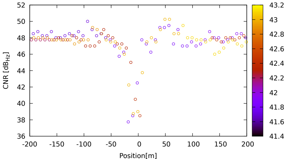
CNR vs position for C33 (B3) on LeicaGS18 - DOY 263 jam. 1
