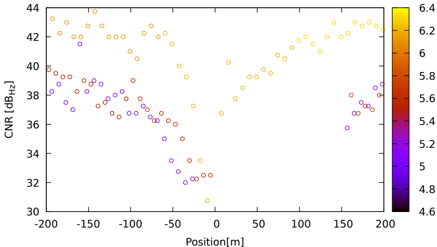
CNR vs position for E09 (E5a) on LeicaGS18 - DOY 263 jam. 1
