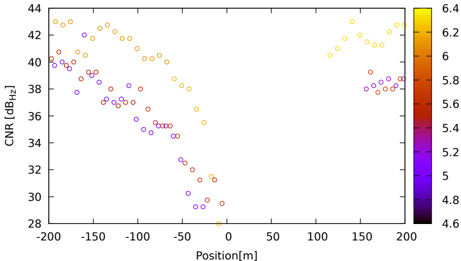
CNR vs position for E09 (E5b) on LeicaGS18 - DOY 263 jam. 1
