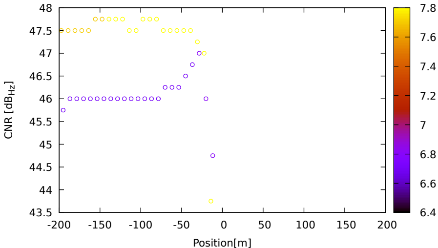
CNR vs position for E09 (E5b) on LeicaGS18 - DOY 263 jam. 2
