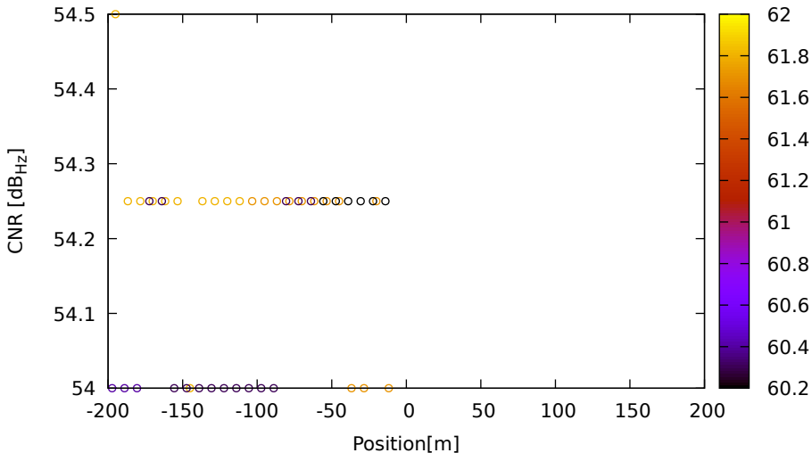
CNR vs position for E12 (E5) on LeicaGS18 - DOY 263 jam. 2
