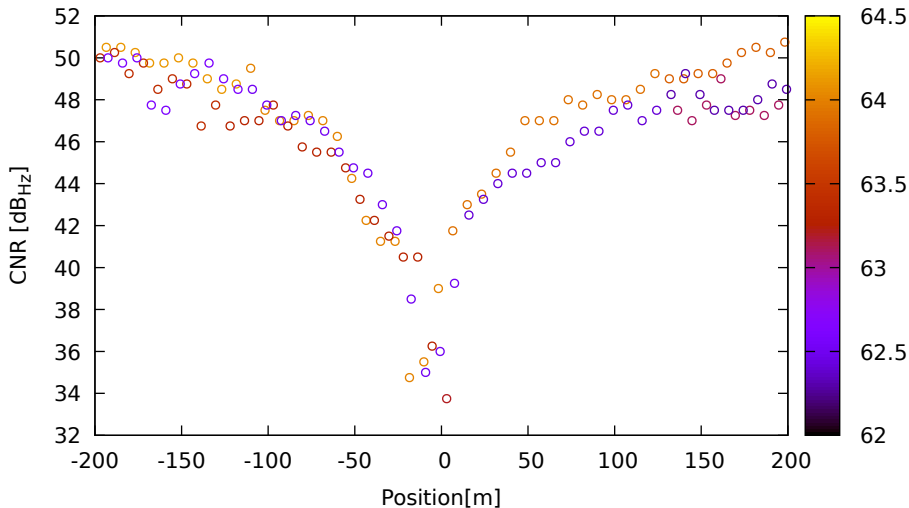
CNR vs position for E12 (E5b) on LeicaGS18 - DOY 263 jam. 1
