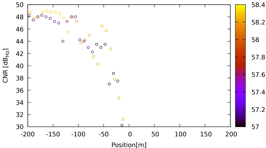
CNR vs position for E19 (E1) on LeicaGS18 - DOY 263 jam. 2
