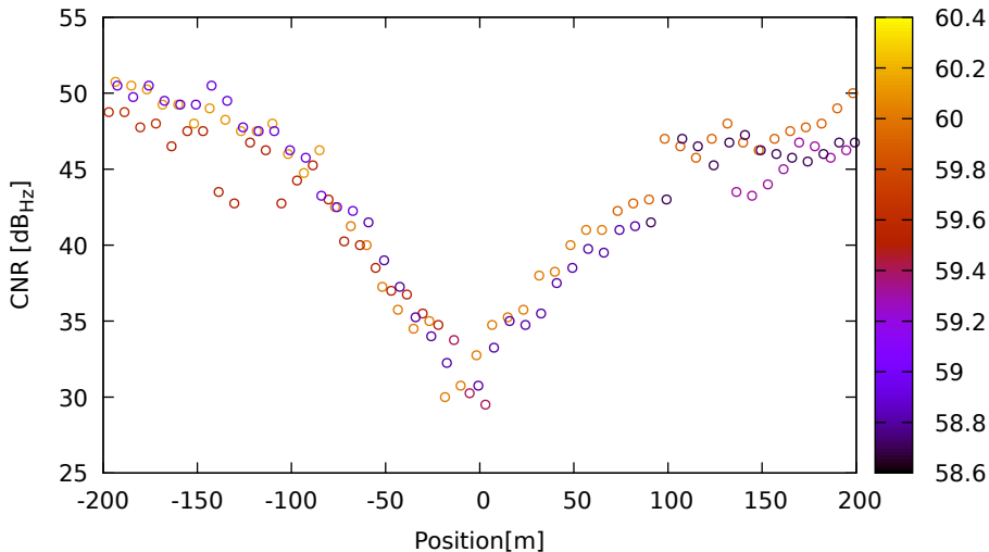
CNR vs position for E19 (E5) on LeicaGS18 - DOY 263 jam. 1
