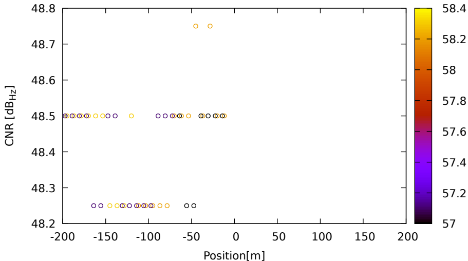
CNR vs position for E19 (E5b) on LeicaGS18 - DOY 263 jam. 2
