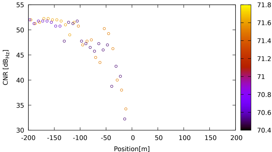
CNR vs position for G03 (L2) on LeicaGS18 - DOY 263 jam. 2
