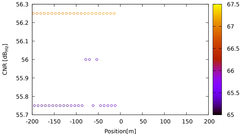
CNR vs position for G04 (L5) on LeicaGS18 - DOY 263 jam. 2
