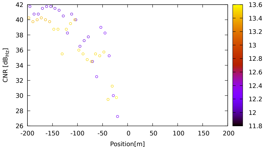
CNR vs position for G06 (L1) on LeicaGS18 - DOY 263 jam. 2
