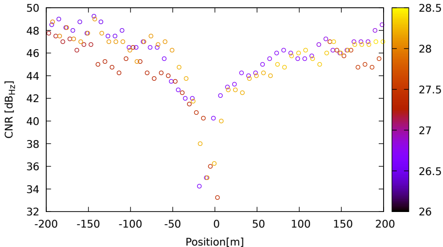
CNR vs position for G09 (L5) on LeicaGS18 - DOY 263 jam. 1
