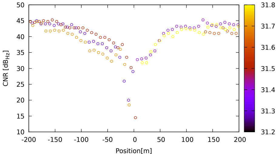
CNR vs position for G19 (L2) on LeicaGS18 - DOY 263 jam. 1
