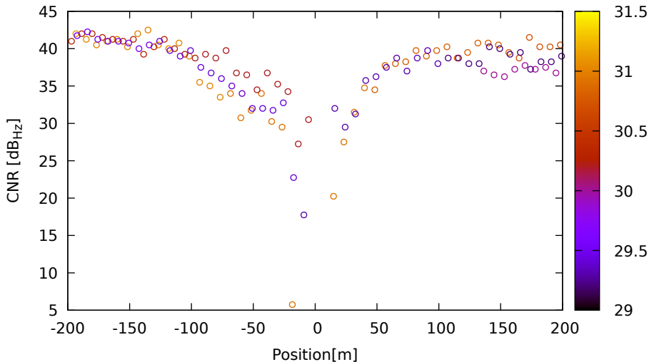
CNR vs position for G21 (L2) on LeicaGS18 - DOY 263 jam. 1
