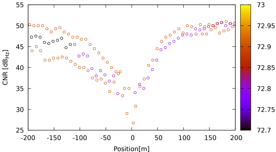
CNR vs position for R02 (G1) on LeicaGS18 - DOY 263 jam. 1
