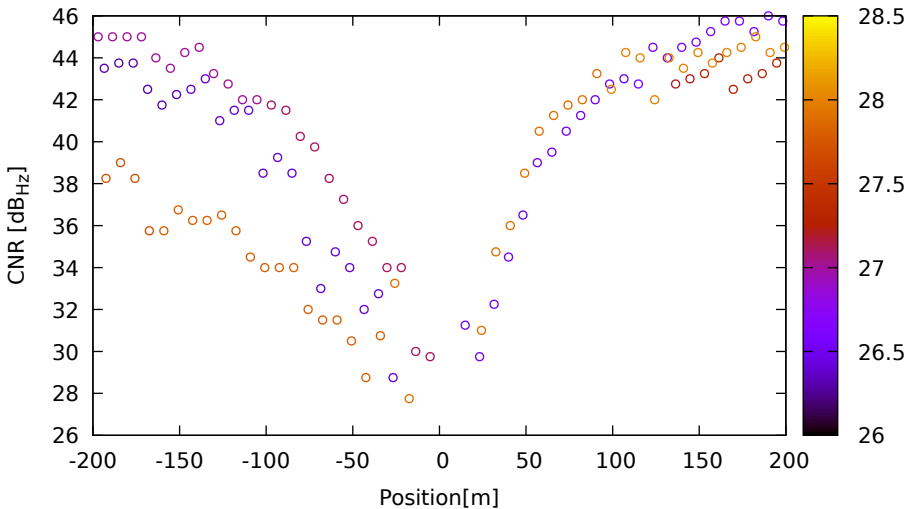
CNR vs position for R03 (G1) on LeicaGS18 - DOY 263 jam. 1
