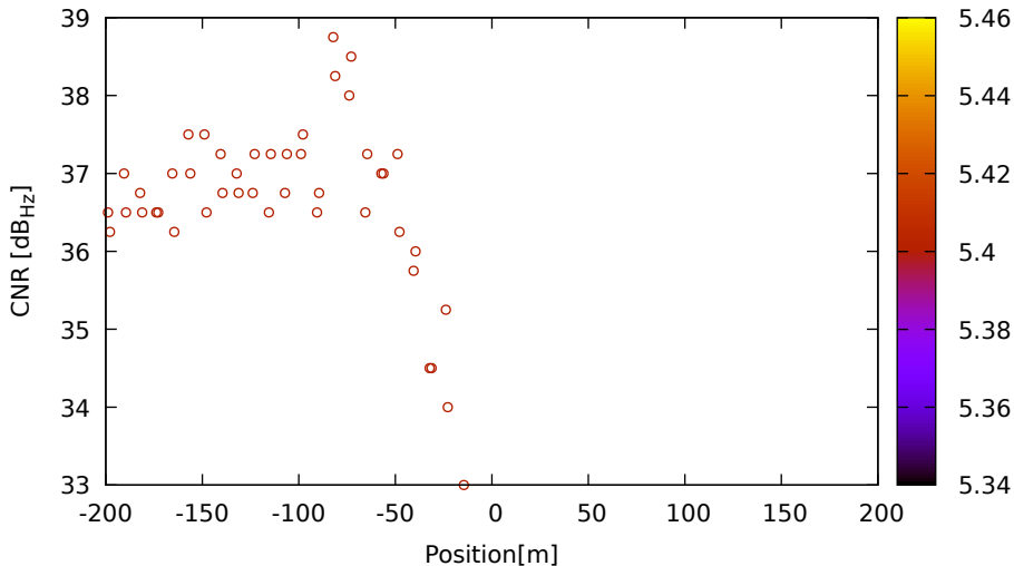
CNR vs position for C02 (B3) on LeicaGS18 - DOY 263 jam. 1
