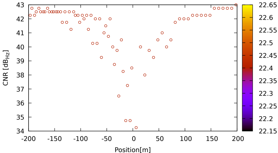
CNR vs position for C05 (B1) on LeicaGS18 - DOY 263 jam. 3
