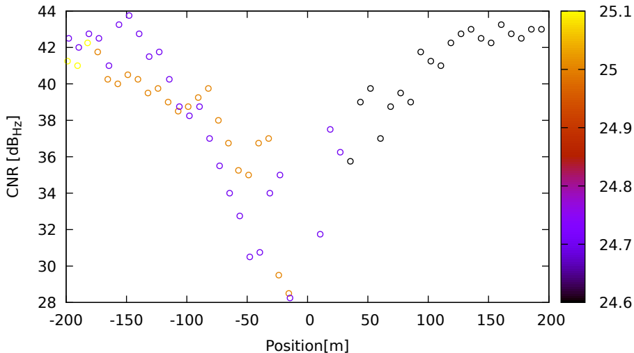
CNR vs position for C06 (B1) on LeicaGS18 - DOY 263 jam. 1
