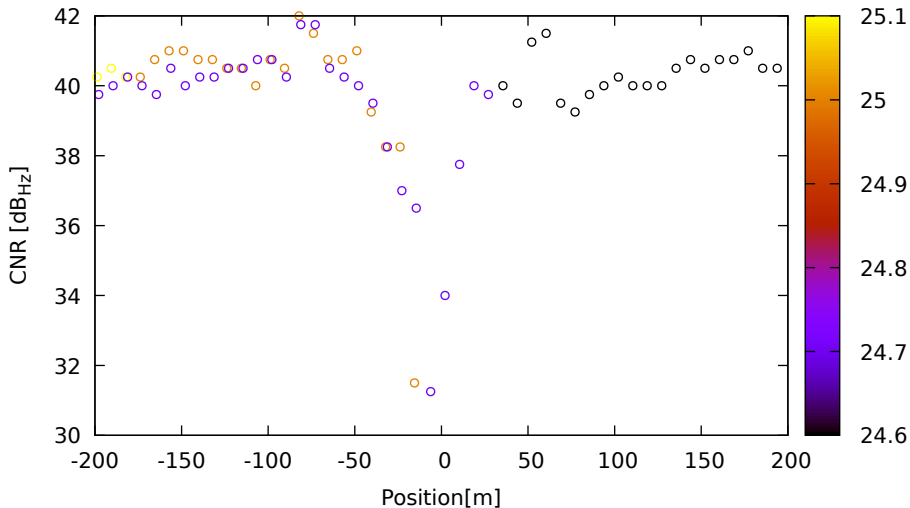
CNR vs position for C06 (B3) on LeicaGS18 - DOY 263 jam. 1
