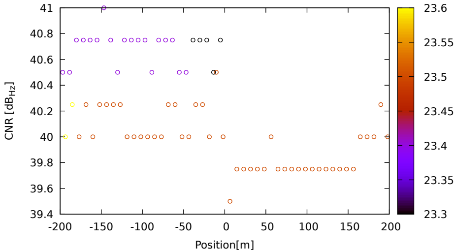
CNR vs position for C06 (B3) on LeicaGS18 - DOY 263 jam. 3
