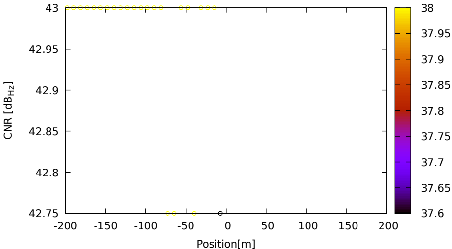
CNR vs position for C09 (B3) on LeicaGS18 - DOY 263 jam. 2
