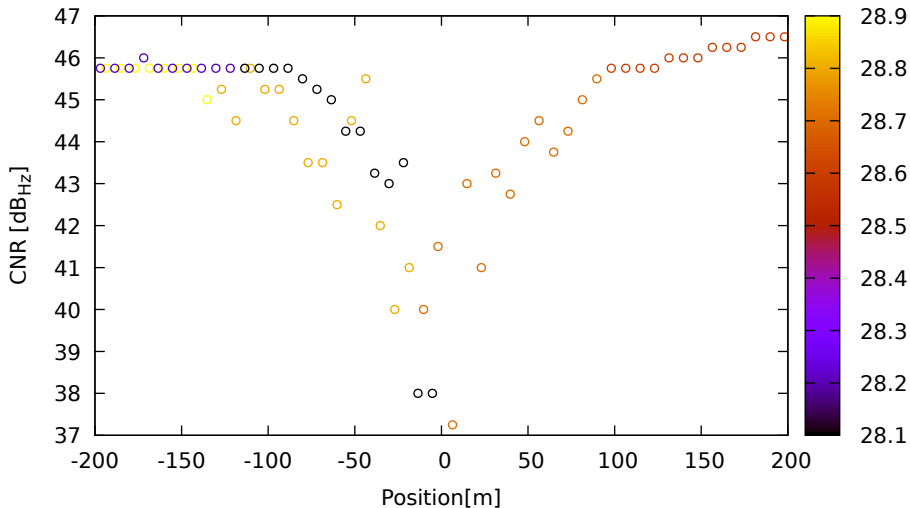
CNR vs position for C11 (B1) on LeicaGS18 - DOY 263 jam. 3
