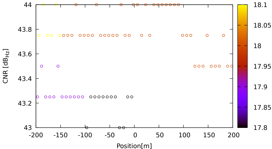
CNR vs position for C16 (B2) on LeicaGS18 - DOY 263 jam. 3
