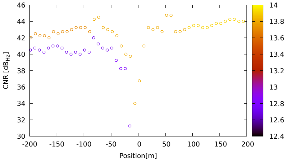
CNR vs position for C26 (B3) on LeicaGS18 - DOY 263 jam. 1
