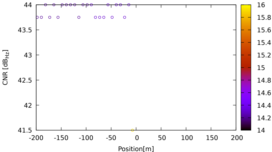
CNR vs position for C26 (B3) on LeicaGS18 - DOY 263 jam. 2
