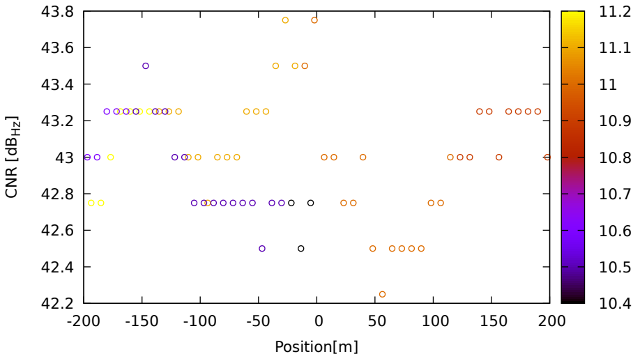
CNR vs position for C34 (B3) on LeicaGS18 - DOY 263 jam. 3
