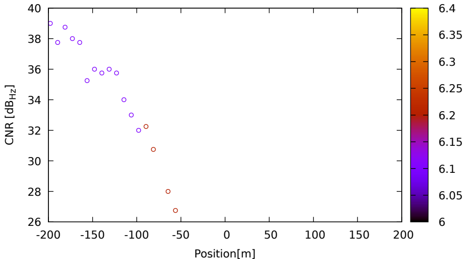
CNR vs position for E09 (E1) on LeicaGS18 - DOY 263 jam. 1
