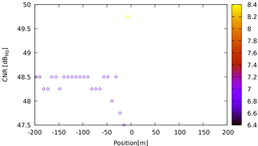
CNR vs position for E09 (E5) on LeicaGS18 - DOY 263 jam. 2
