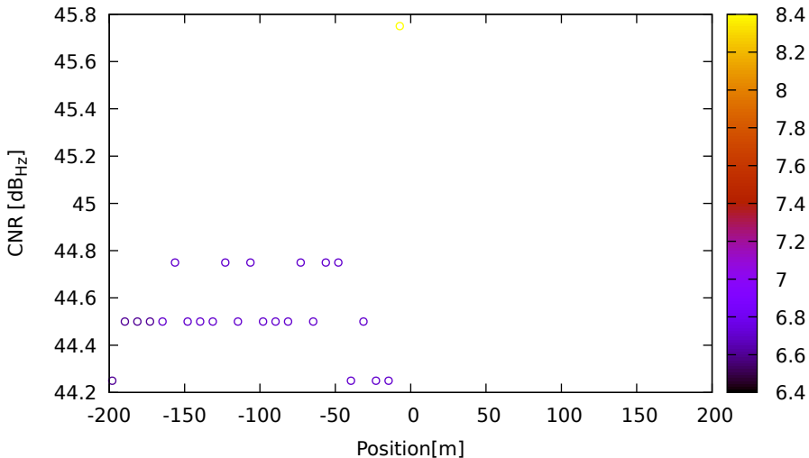
CNR vs position for E09 (E5a) on LeicaGS18 - DOY 263 jam. 2
