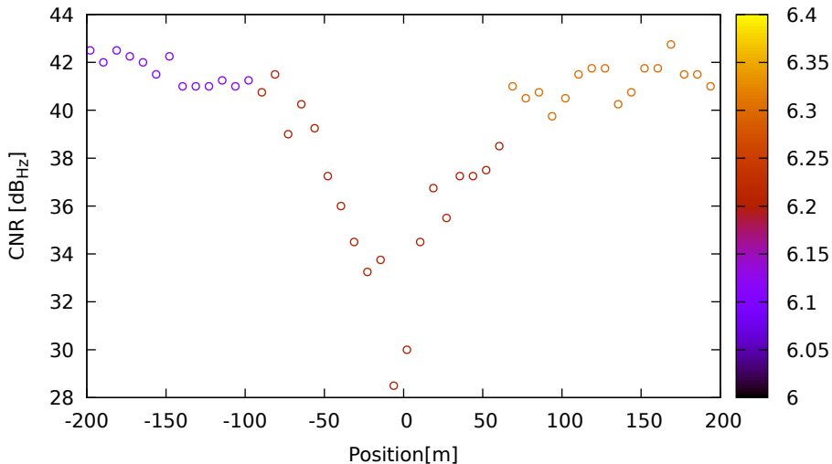
CNR vs position for E09 (E5b) on LeicaGS18 - DOY 263 jam. 1
