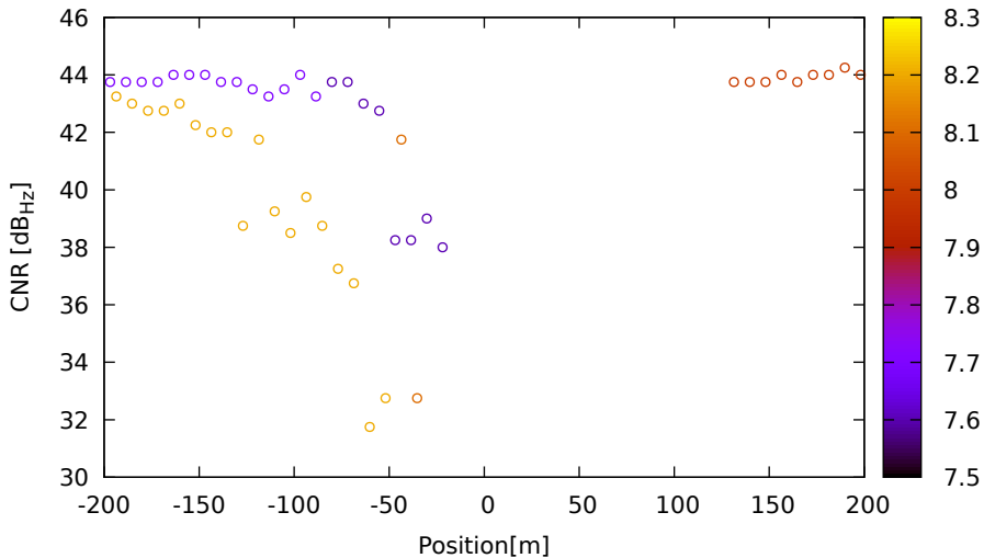
CNR vs position for E33 (E1) on LeicaGS18 - DOY 263 jam. 3
