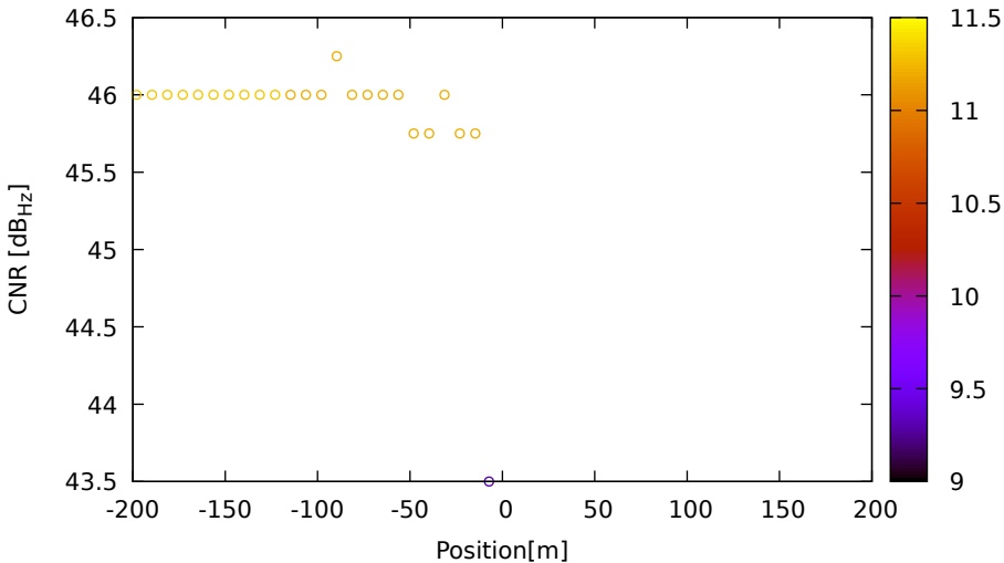
CNR vs position for E33 (E5a) on LeicaGS18 - DOY 263 jam. 2
