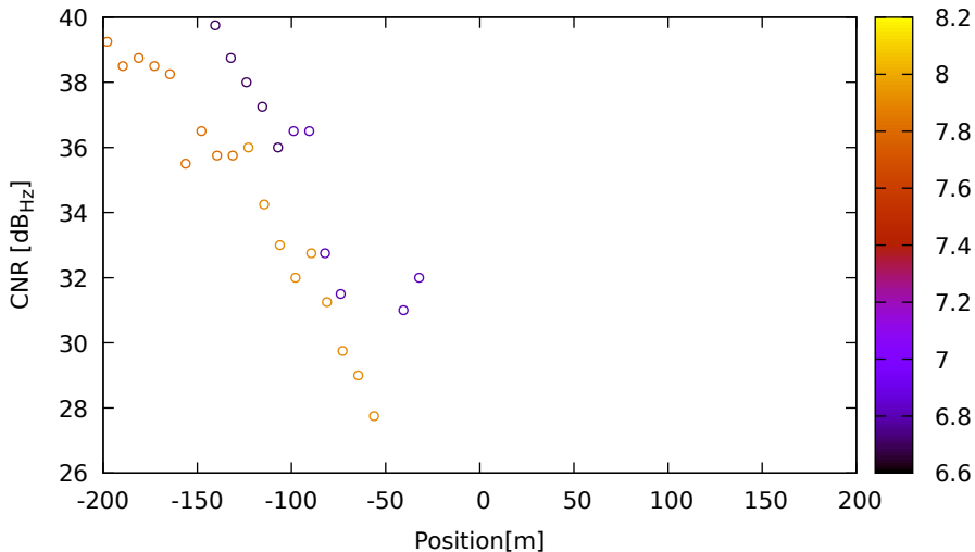
CNR vs position for E36 (E1) on LeicaGS18 - DOY 263 jam. 1
