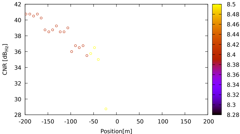
CNR vs position for E36 (E1) on LeicaGS18 - DOY 263 jam. 2
