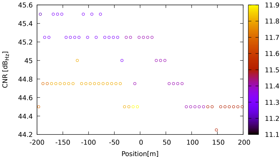
CNR vs position for E36 (E5a) on LeicaGS18 - DOY 263 jam. 3
